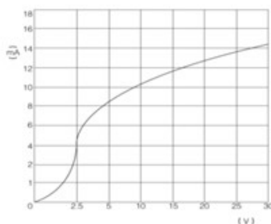
Input Current v. Control Voltage: 4 ~ 32VDC
