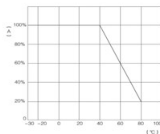
Load Current Derating v. Ambient Temperature
