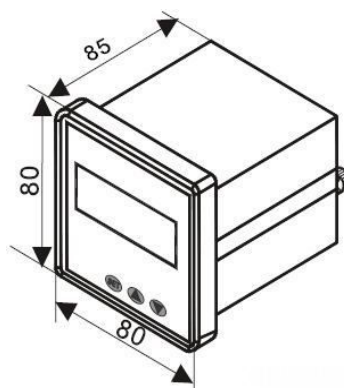
Outline size
