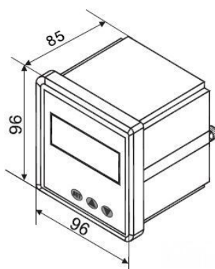
Outline size
