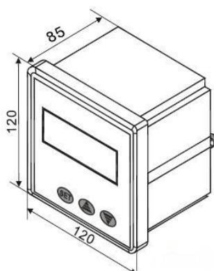
Outline size
